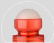
P3004 Volume:50ml Ball Diameter:35.56mm Height:97.6mm Material Cap:PET Bottle:PET Ball:PP
