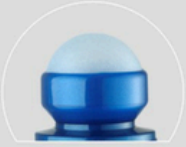
P3003 Volume:50ml Ball Diameter:35.56mm Height:104.6mm Material Cap:PET Bottle:PET Ball:PP
